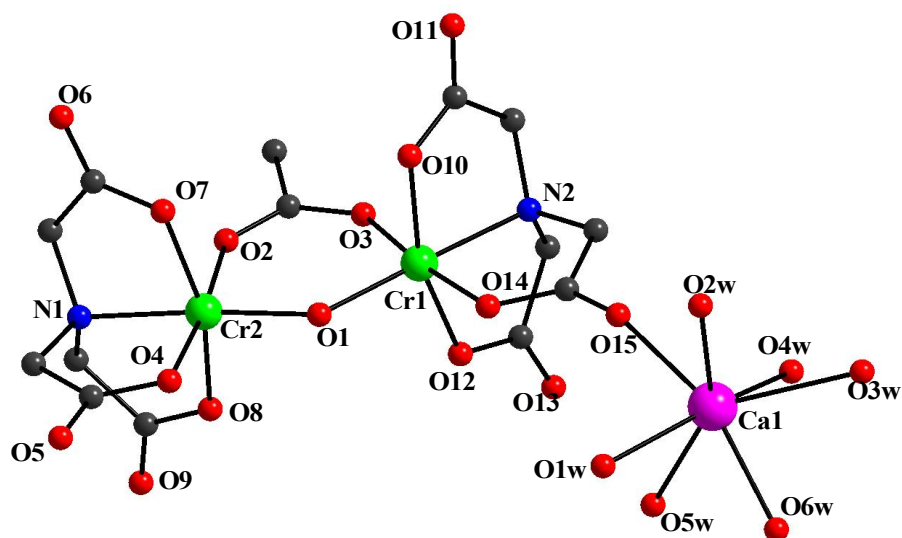
Fig. 1. Structura compusului trinuclear [\text{CaCr}_2(\mu\text{-OH})(\mu\text{-OAc})(\text{nta})_2 \cdot 6\text{H}_2\text{O}] \cdot 2\text{H}_2\text{O} .
